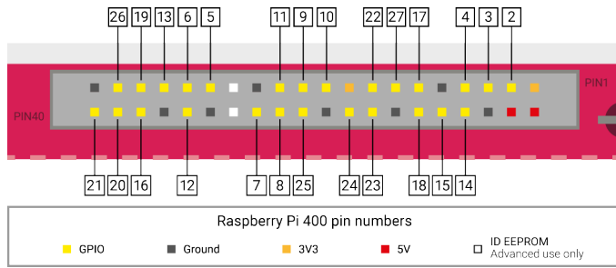
Figure 6-2 Raspberry Pi 400 GPIO pinout
