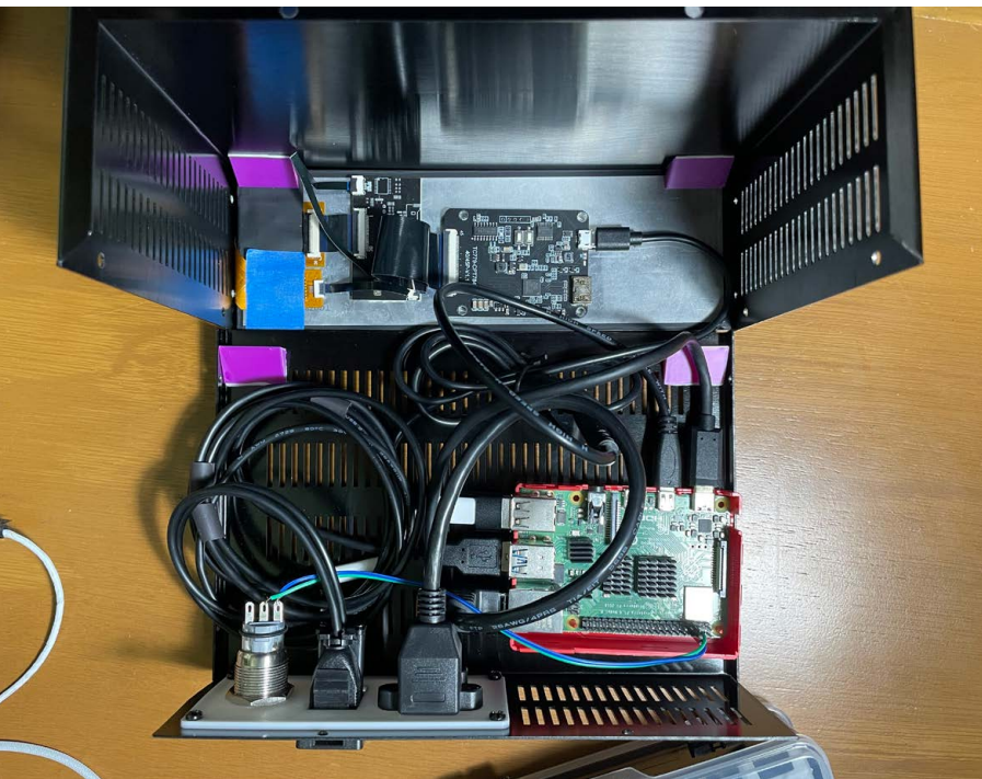
▲ A Raspberry Pi 4 forms the heart of this build. It is connected to a generic 7.9-inch touchscreen display. Extension cables allow for rear ports
