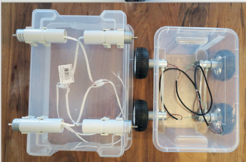
Above The Discoverer is loosely based on Ingmar’s earlier cardboard car ( magpi.cc/1VQv8QJ ), which has live video streaming
