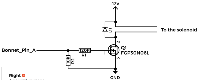
Right A general-purpose low-side driver circuit
